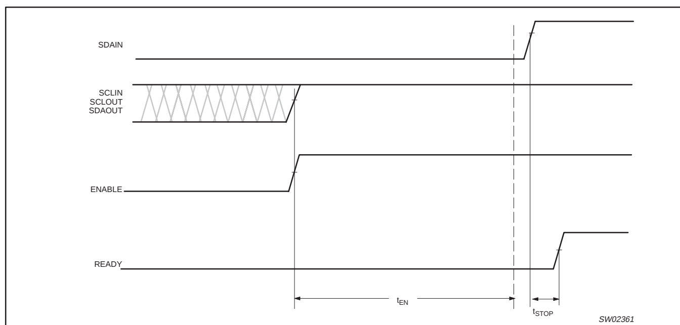
Figure 15. t_{\text{STOP}} that can occur after t_{\text{ENABLE}}
