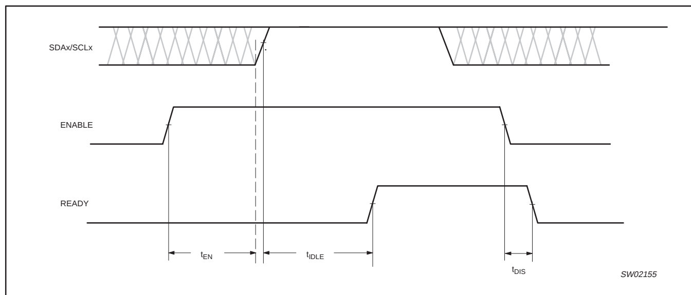
Figure 14. Timing for t_{\text{ENABLE}} , t_{\text{IDLE}} , and t_{\text{DISABLE}}
