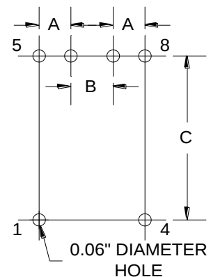
Board Layout
