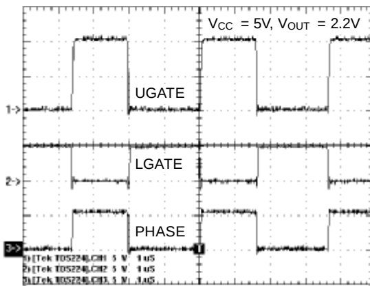
Bootstrap Wave Form
