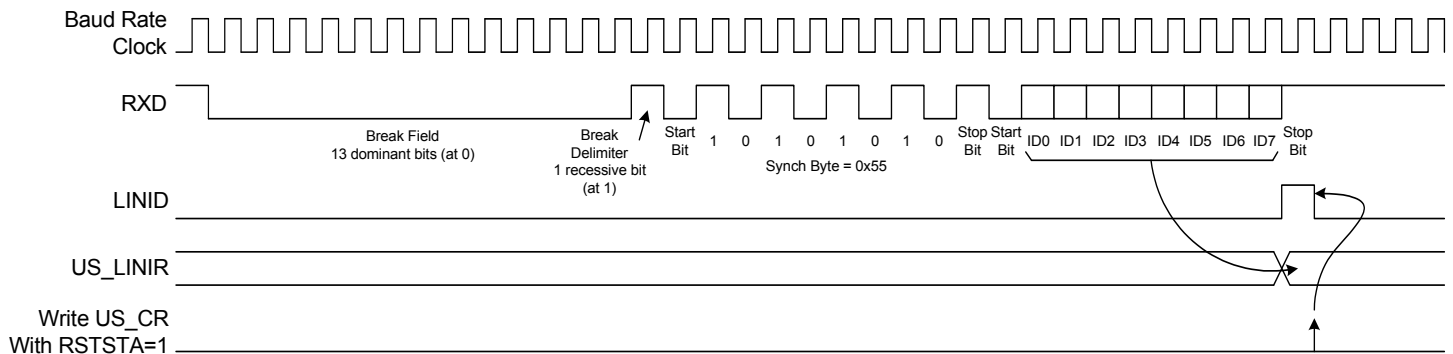
Figure 25-28. Header Reception
