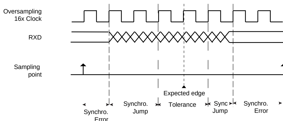
Figure 25-47. Bit Resynchronization
