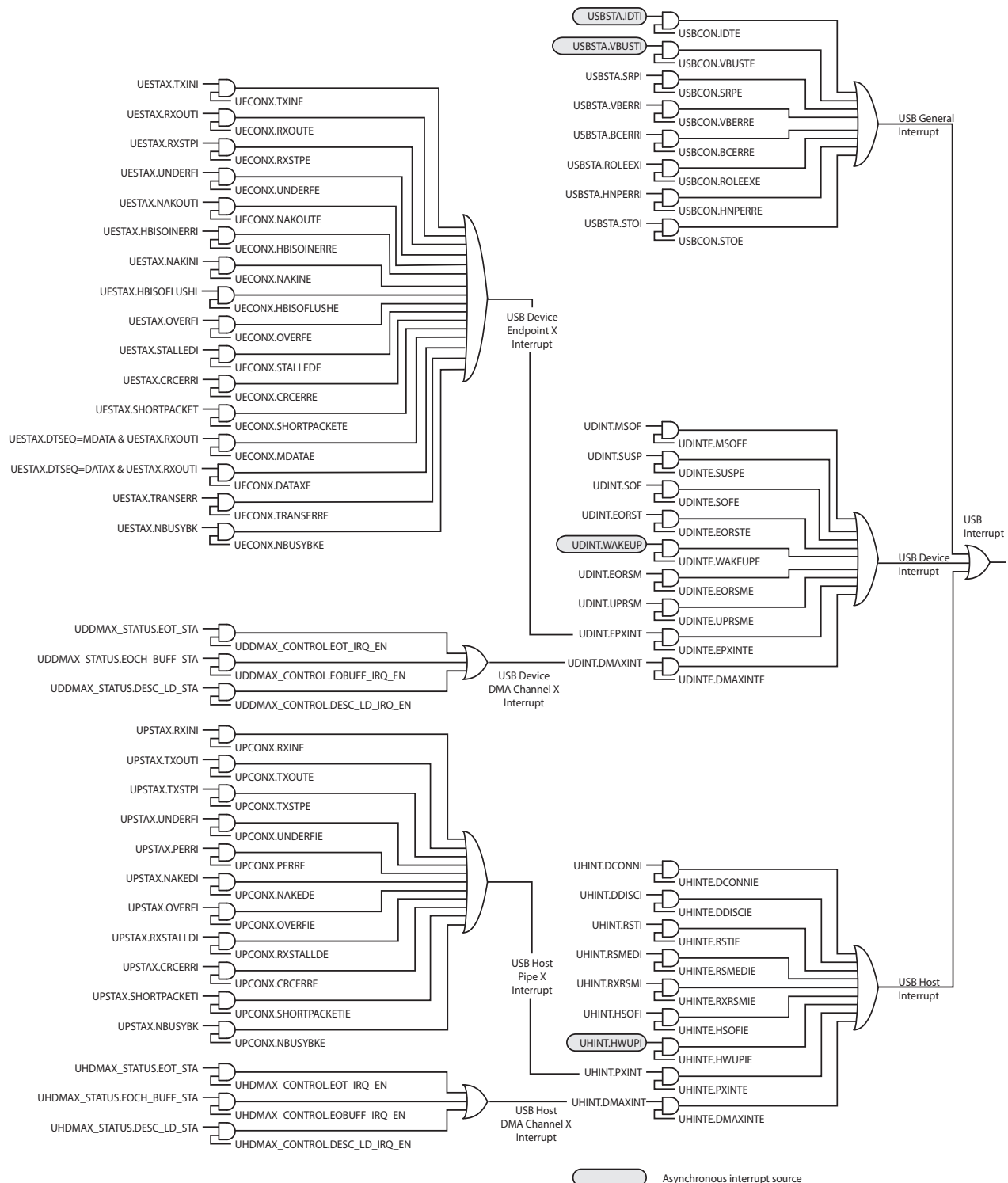
Figure 27-6. Interrupt System
