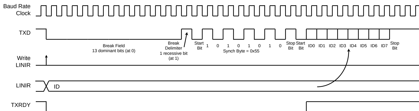
Figure 25-27. Header Transmission
