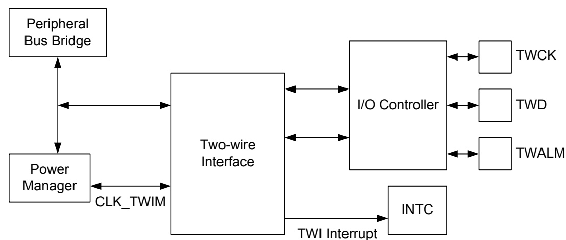
Figure 23-1. Block Diagram
