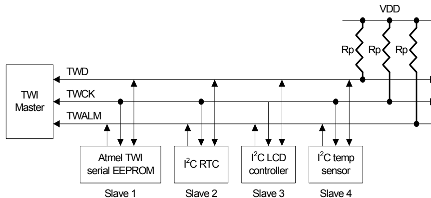
Figure 23-2. Application Block Diagram
