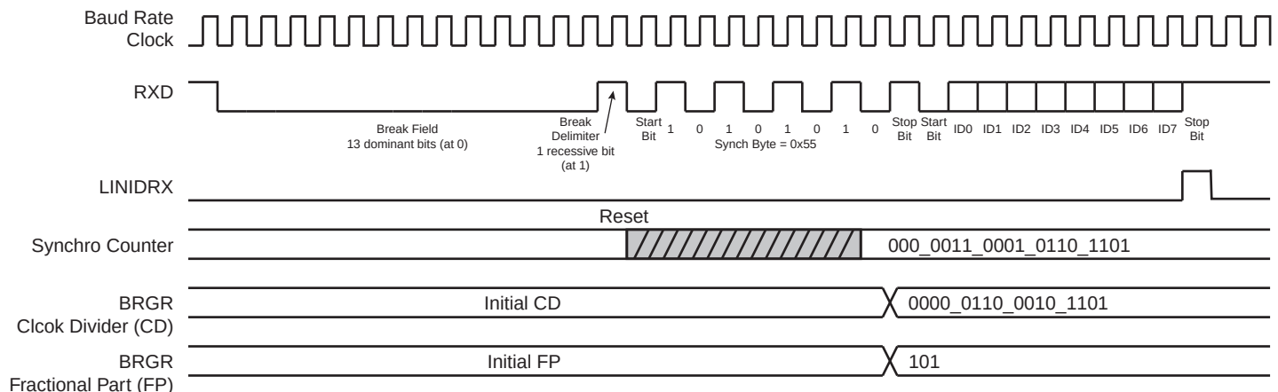
Figure 25-30. Slave Node Synchronization
