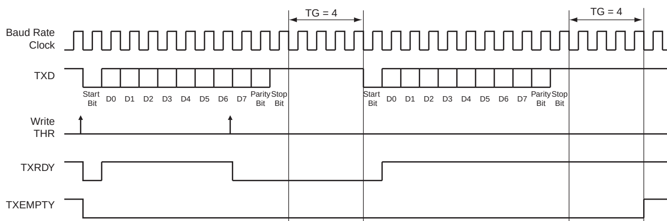
Figure 25-9. Timeguard Operation
