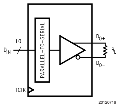
FIGURE 17. V_{OD} Diagram
