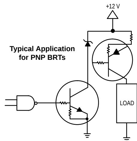
Figure 22. Inexpensive, Unregulated Current Source
