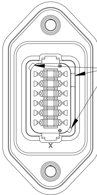
DT04-12PC-LE21 KEY ARR. -C- HOUSING COLOR: GREEN
