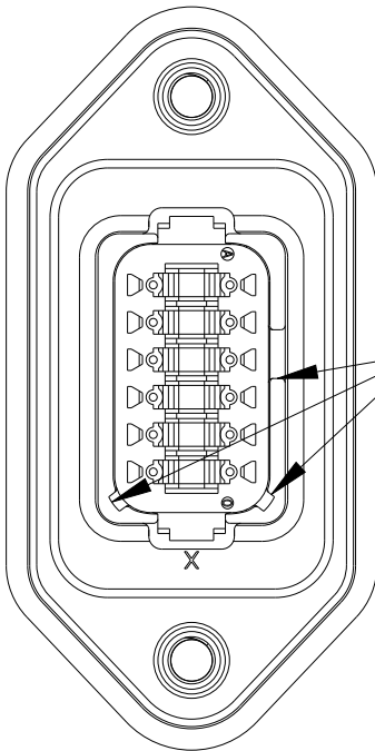
DT04-12PB-LE21 KEY ARR. -B- HOUSING COLOR: BLACK
