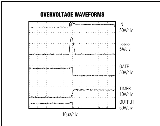
Figure 11. Overvoltage Waveforms
