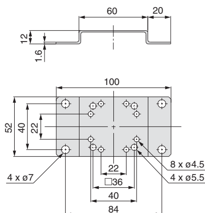
Flat bracket
