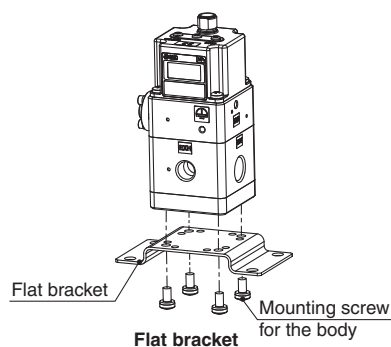
Flat bracket
