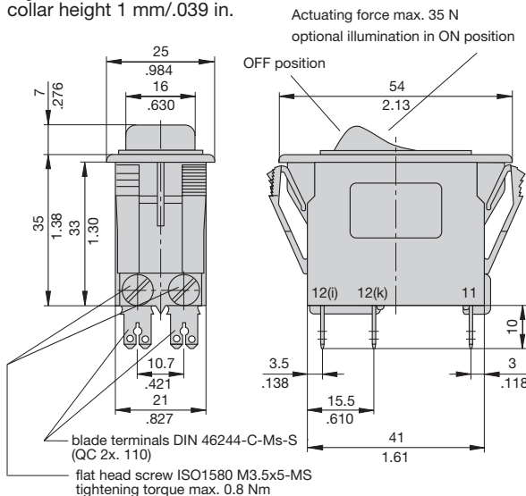
Style F3.1 collar height 1 mm/.039 in.
