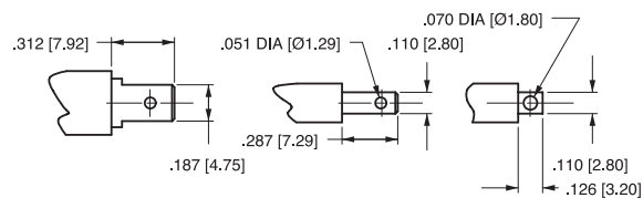
SOLDER TYPE
