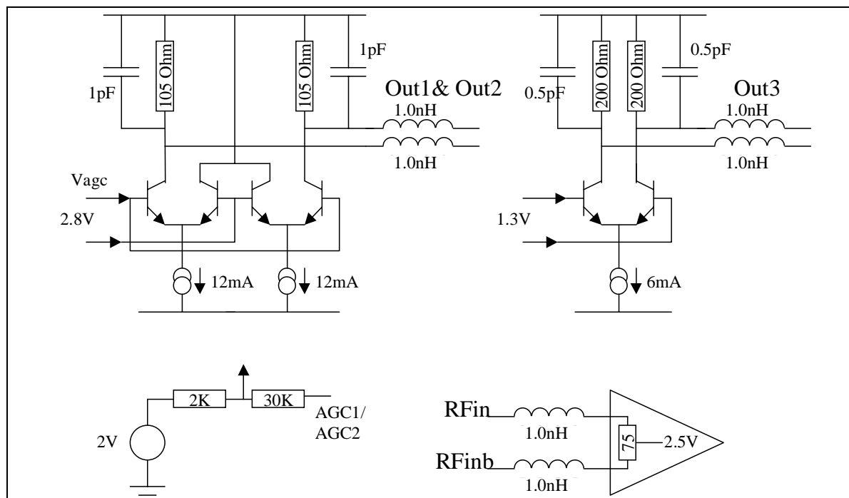
Figure 5 - ZL40000 I/O Circuits
