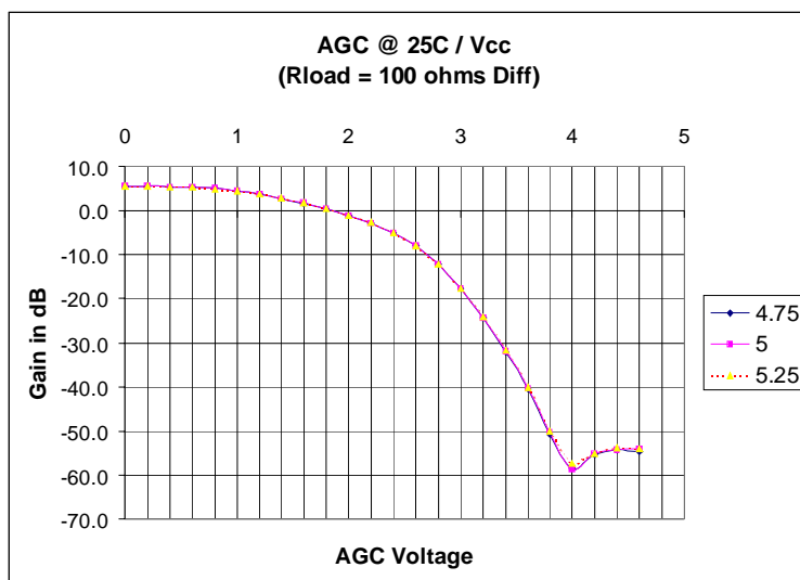
Figure 12 - Typical AGC / VCC @ 25C
