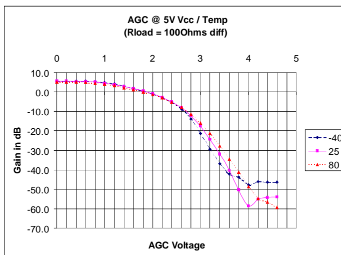
Figure 13 - Typical AGC / Temp @ 5 V Vcc
