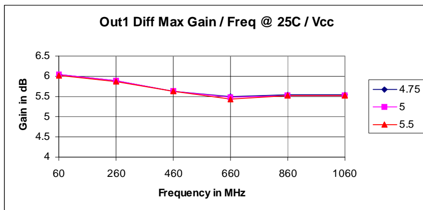
Figure 6 - Typical Ch1&2 Diff Gain / Freq / Vcc @ 25C
