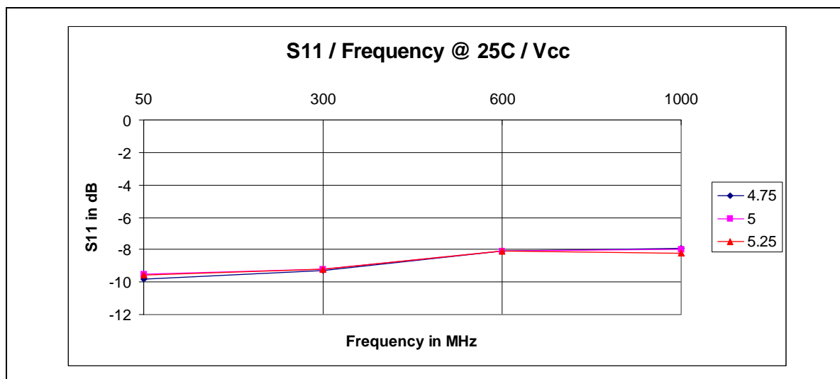
Figure 36 - Typical S11 in 50Ohm System
