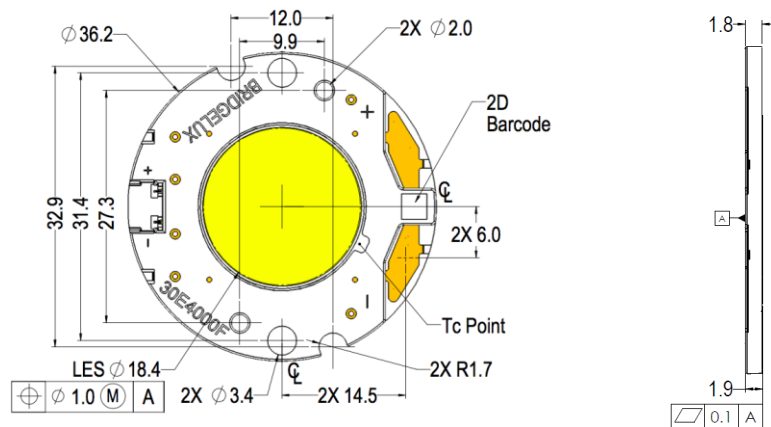
Figure 9: Drawing for Vero 18 LED Array
