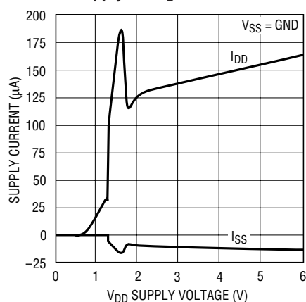
Quiescent Supply Currents vs Supply Voltage
