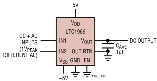
\pm 5V Supplies, Differential, DC-Coupled RMS-to-DC Converter
