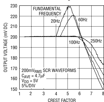
Performance vs Large Crest Factors
