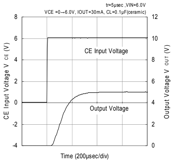
XC6215B502
