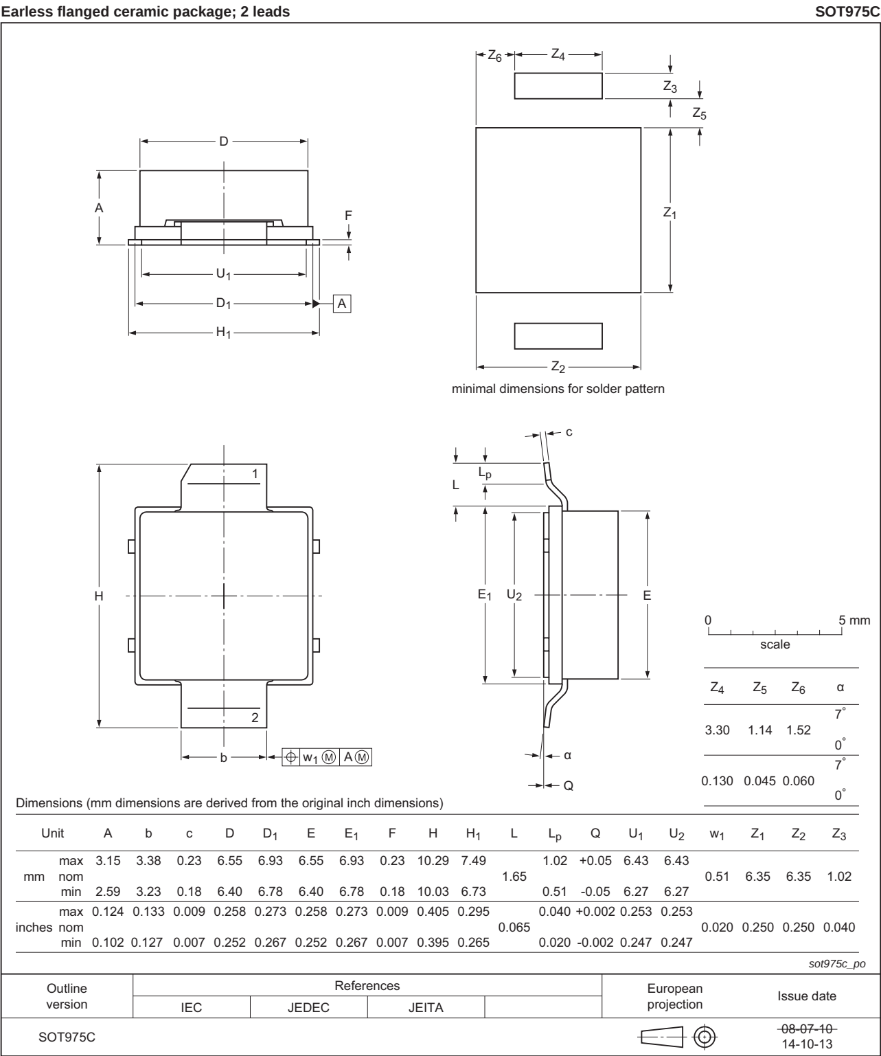
Fig 13. Package outline SOT975C
