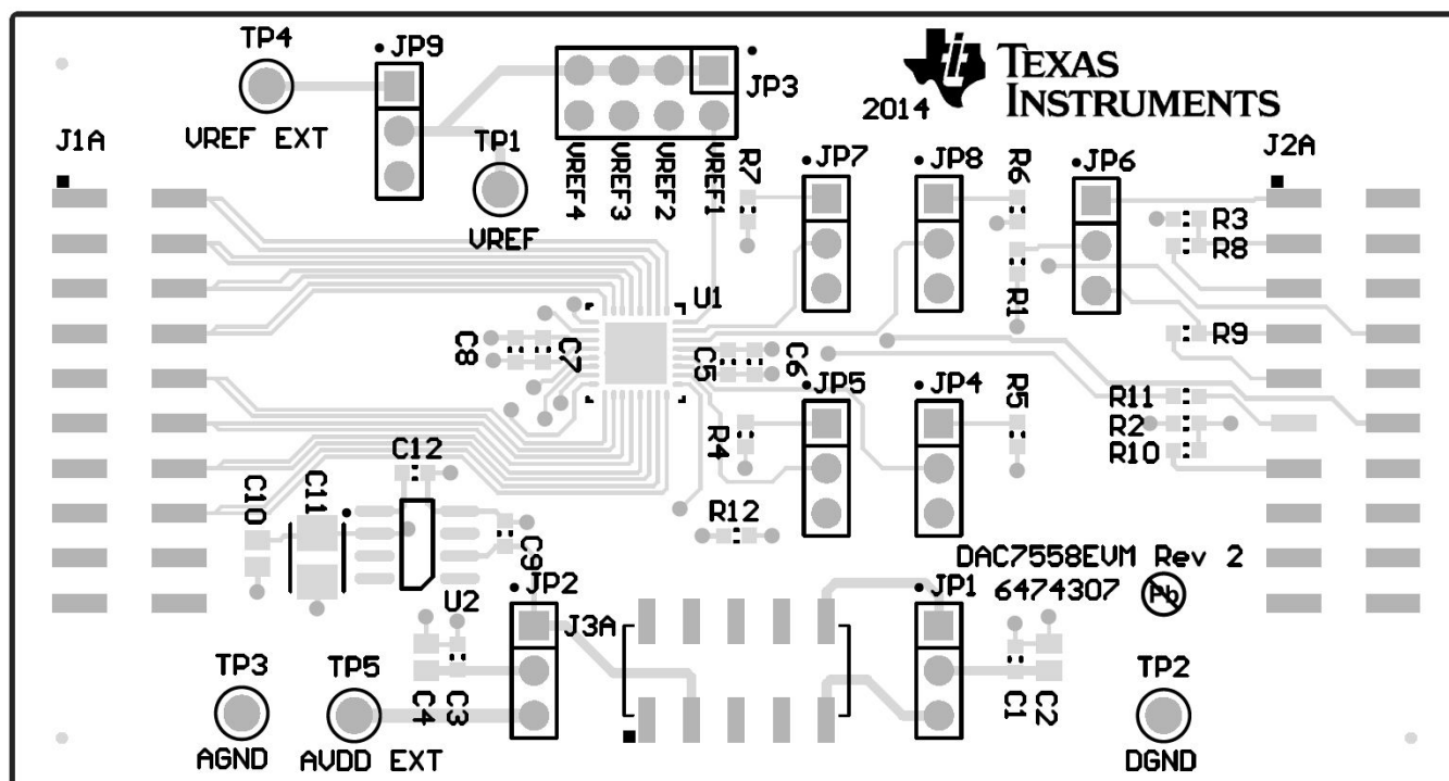
Figure 3. DAC7558EVM PCB Top Layer Layout
