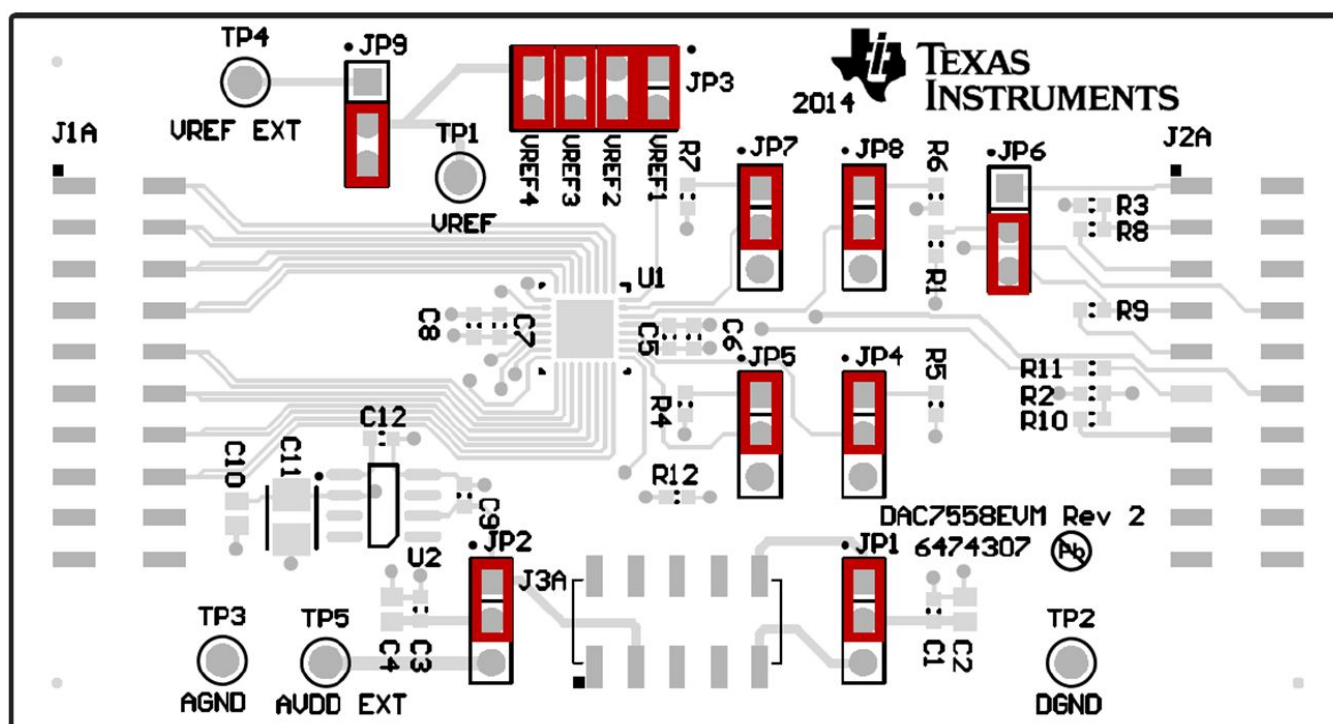
Figure 1. Default Jumper Placement for the DAC7558EVM
