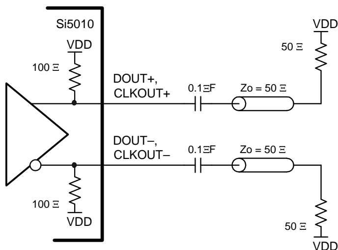
Figure 9. Output Termination for DOUT and CLKOUT (AC-coupled)
