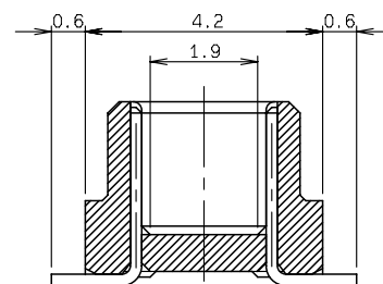
SECT. D-D
