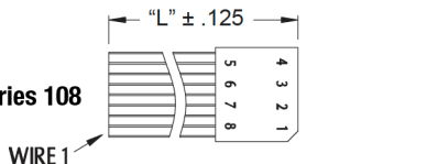
Cable Detail
