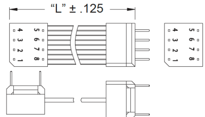
Cable Detail
