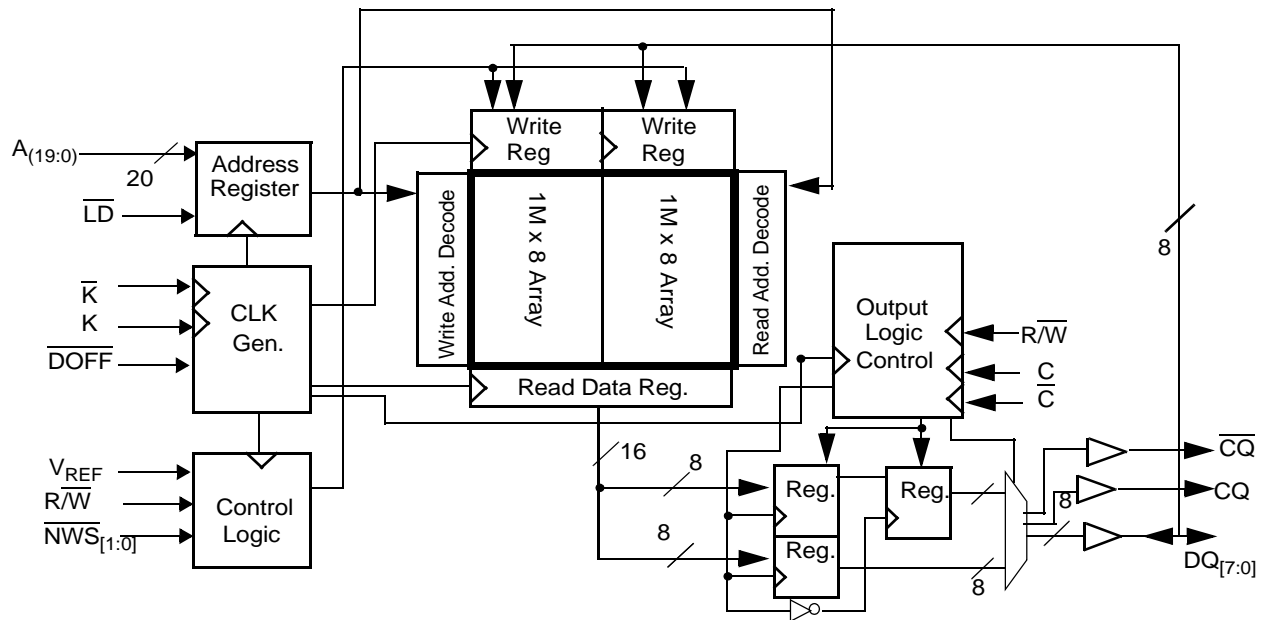
Logic Block Diagram (CY7C1316BV18)
