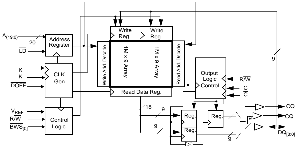
Logic Block Diagram (CY7C1916BV18)
