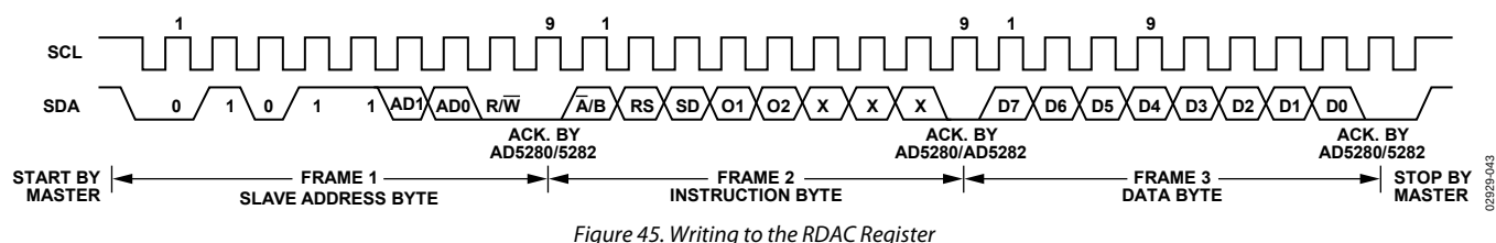
Figure 45. Writing to the RDAC Register
