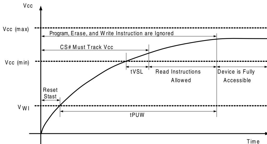
Figure 9.1 Power-up Timing
