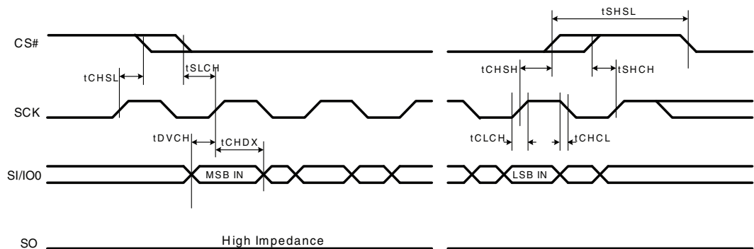
Figure 9.4 Input Timing
