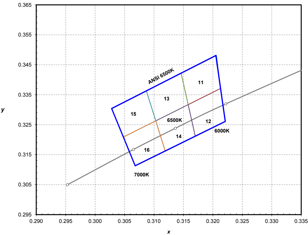
Figure 21. ANSI 6500K 1/6th color bin structure, forward current = 100 mA, thermal pad temperature = 25°C.
