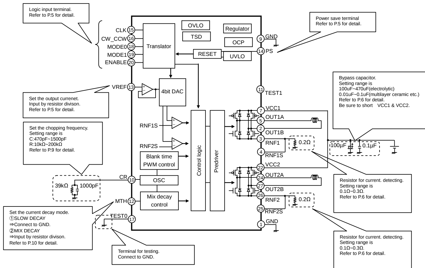
Figure.8 Block diagram &amp; Application circuit diagram
