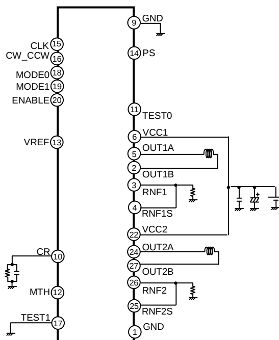
Figure 1. BD63510EFV application circuit diagram
