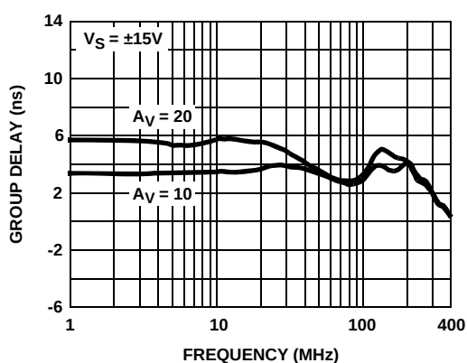
FIGURE 28. GROUP DELAY
