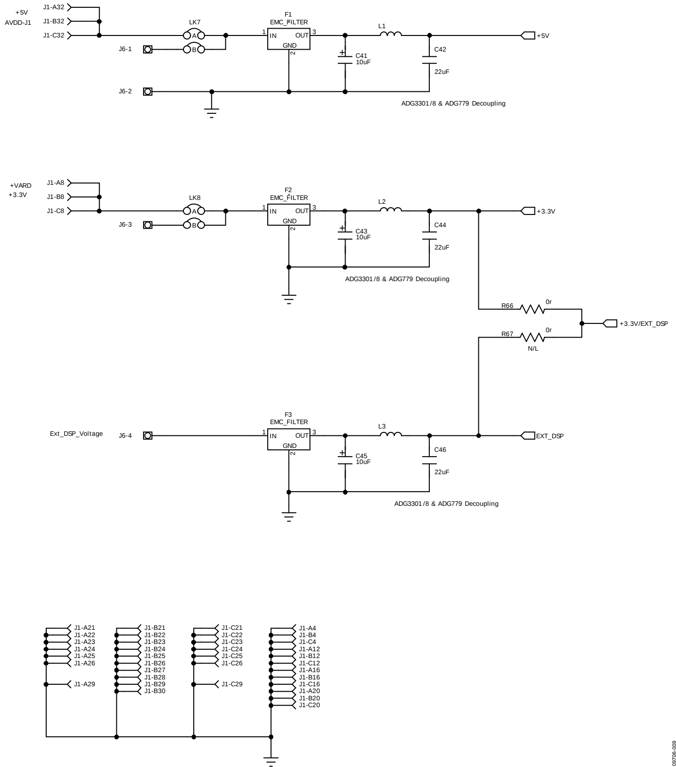
Figure 9. EVAL-AD7280EDZ Schematic—Page 4
