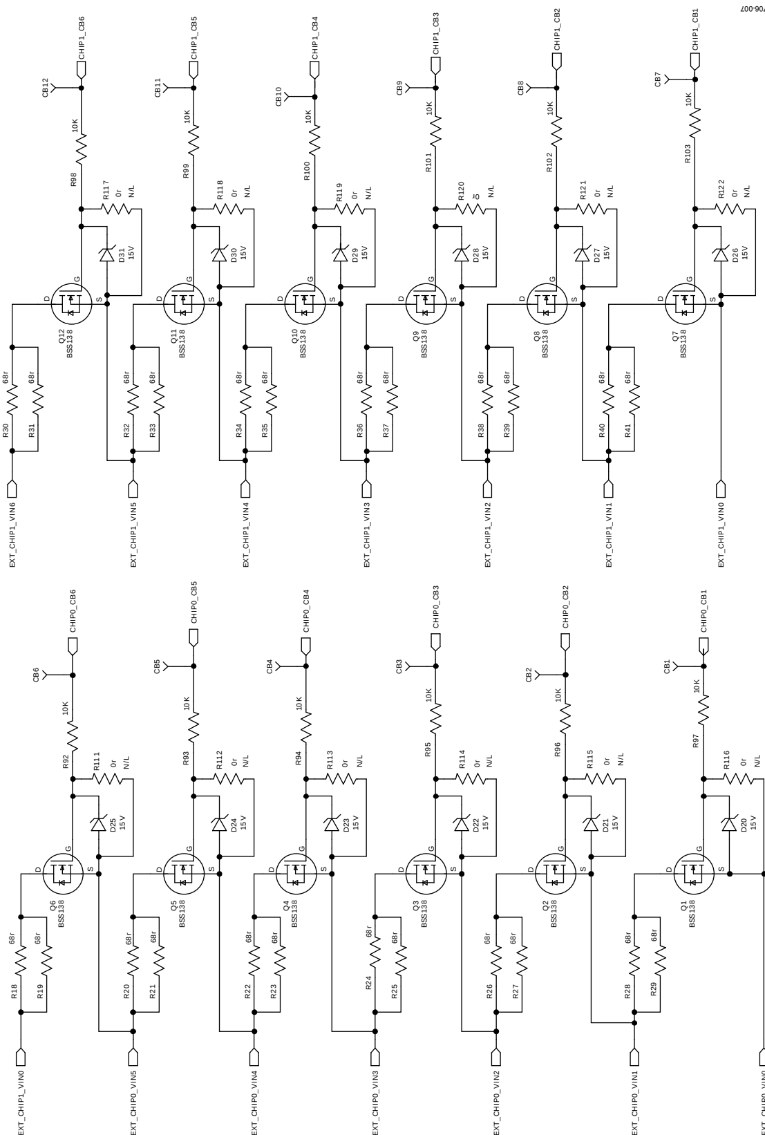
Figure 7. EVAL-AD7280AEDZ Schematic—Page 2
