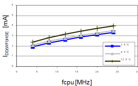
Figure 14. Typ. I_{DD(WFI)HSE} vs. f_{CPU} @ V_{DD} = 5.0 V, peripheral = on
