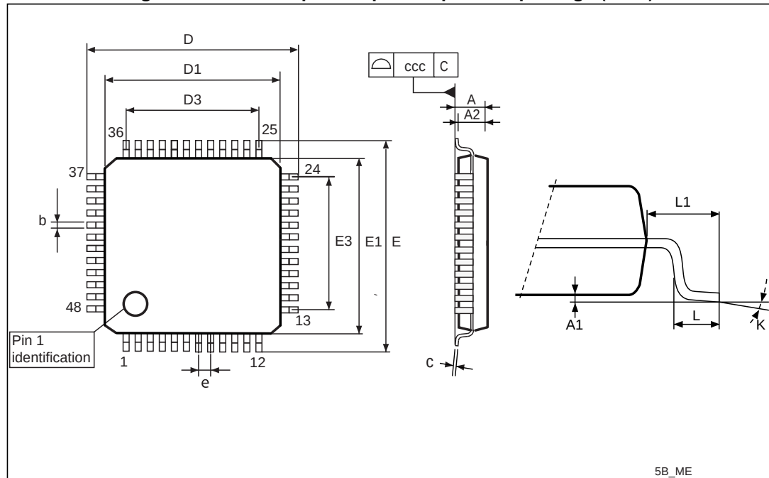
Figure 43. LQFP 48-pin low profile quad flat package (7 x 7)
