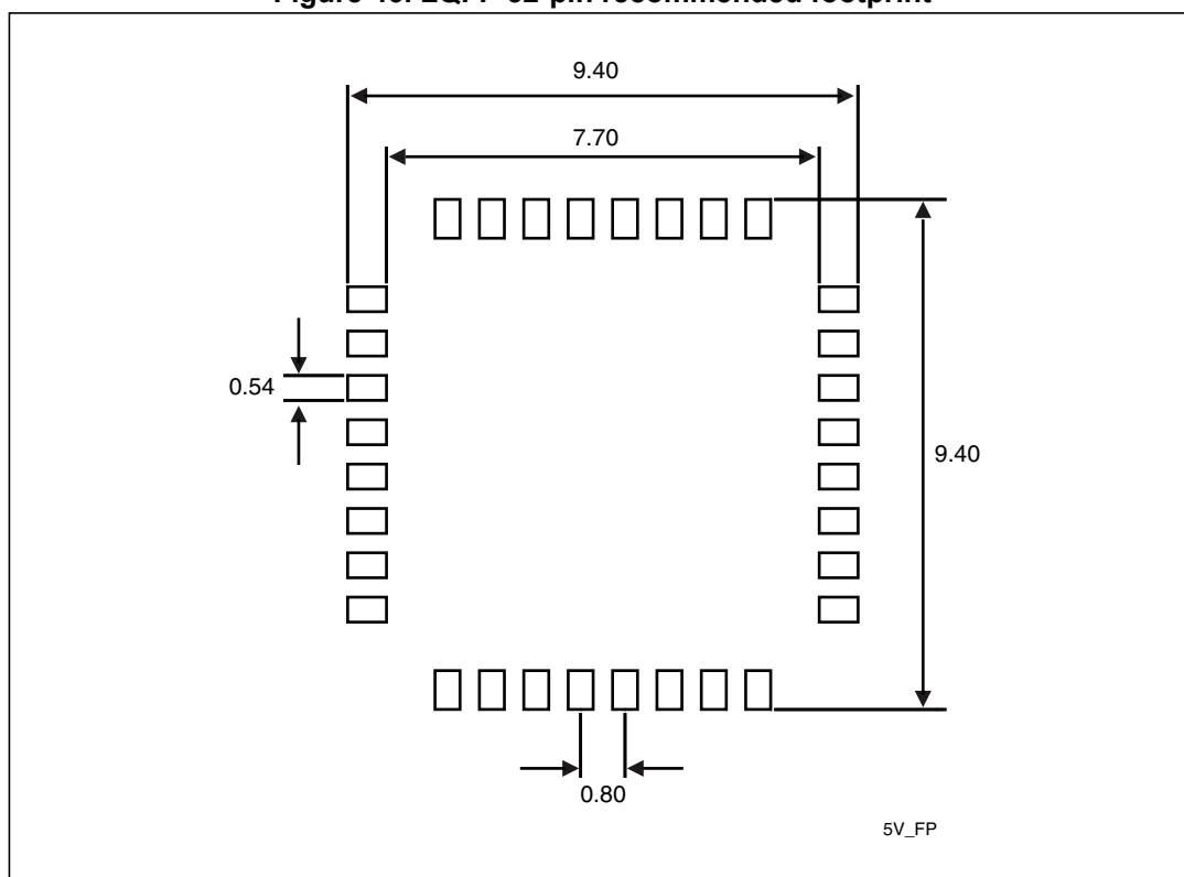
Figure 46. LQFP 32-pin recommended footprint
