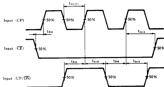
Waveforms showing minimum pulse width for CP, set-up and hold times for CE to CP and UP/DN to CP
