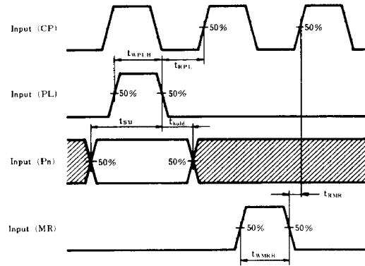
(Fig. 2) t_{WPLH} , t_{RPL} , t_{RMR} , t_{WMRH} , t_{SU}(P_n \rightarrow PL) , t_{hold}(P_n \rightarrow PL)
