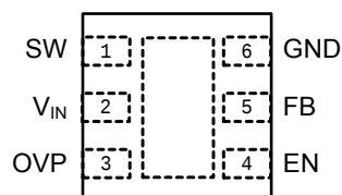
U-DFN2020-6
