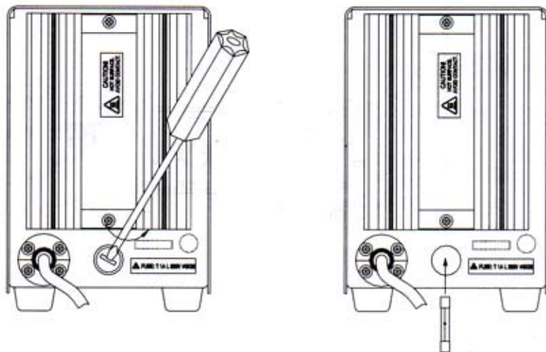
15/18V FUSE
