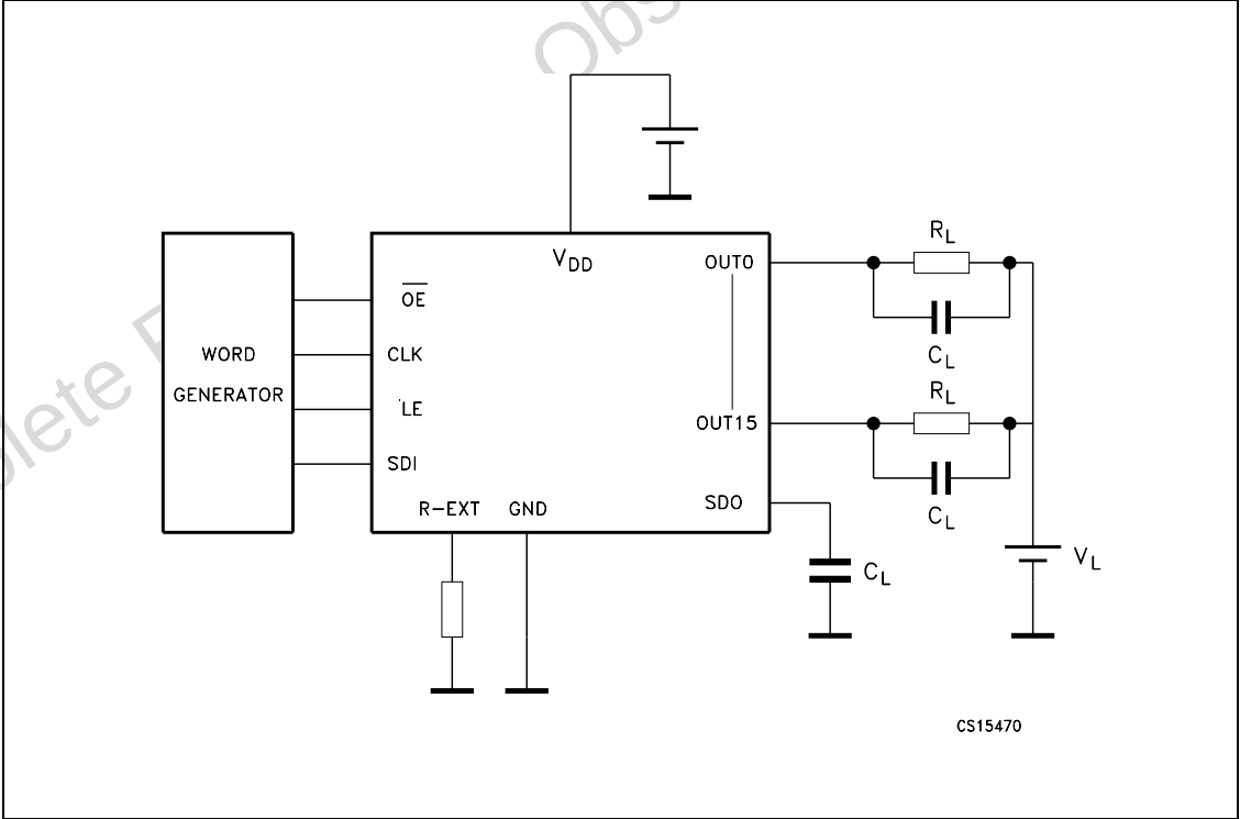
Figure 12. AC characteristics
