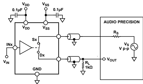
Figure 30. THD + Noise
