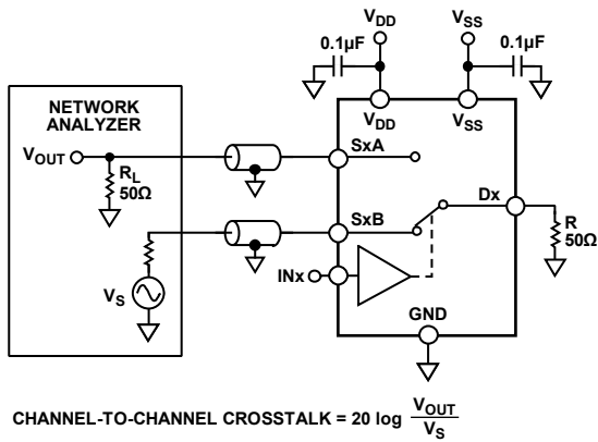
Figure 28. Channel-to-Channel Crosstalk
