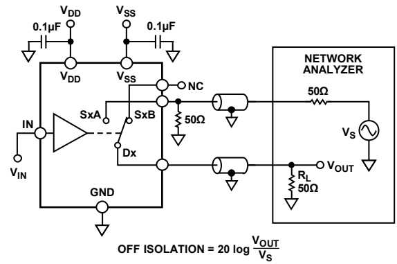
Figure 29. Off Isolation
