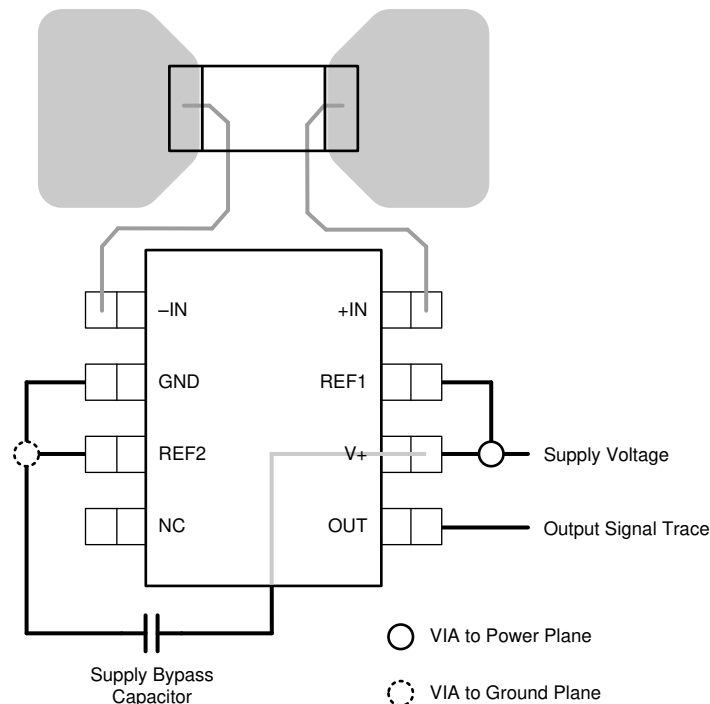
Figure 10-1. Layout Example
