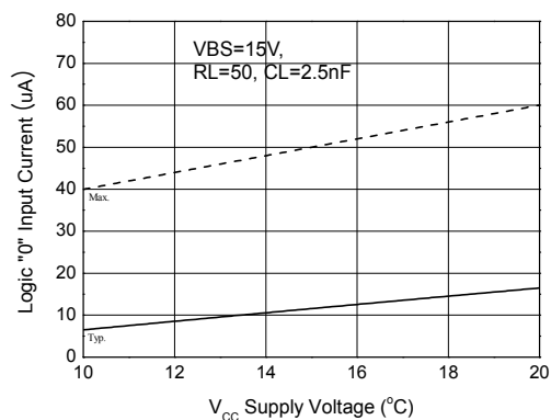
Figure 16b. Logic "0" IN Current vs VCC Supply Voltage
