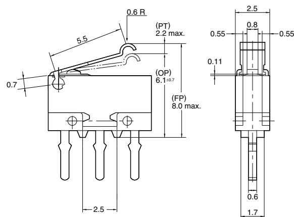
External dimensions
