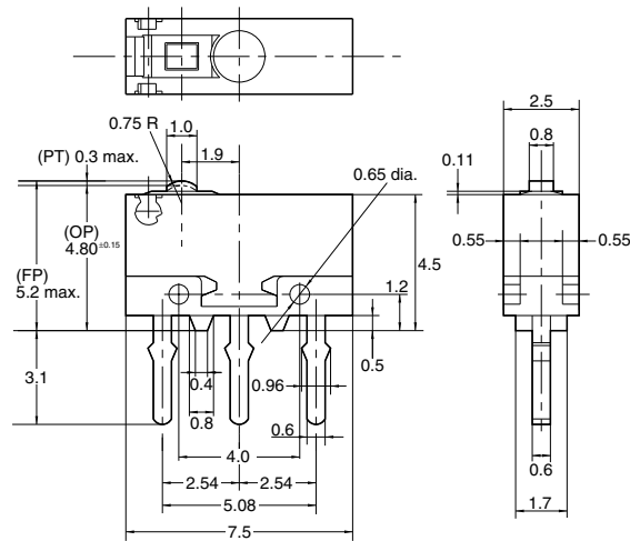
External dimensions
