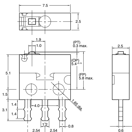
External dimensions
