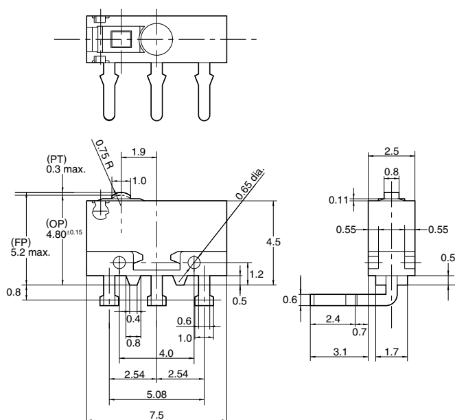
External dimensions
