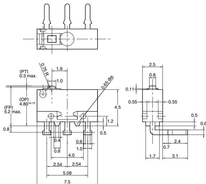
External dimensions
