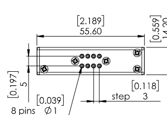
TOP view - solder pins
