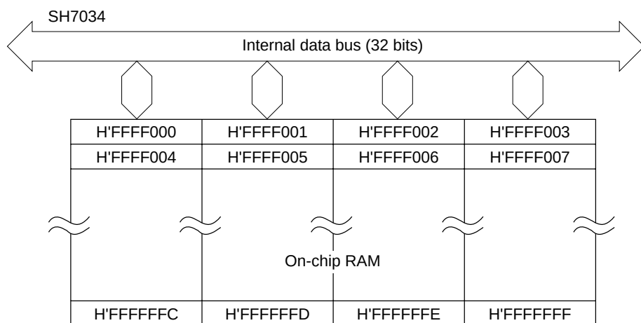
Figure 18.1 Block Diagram of RAM
