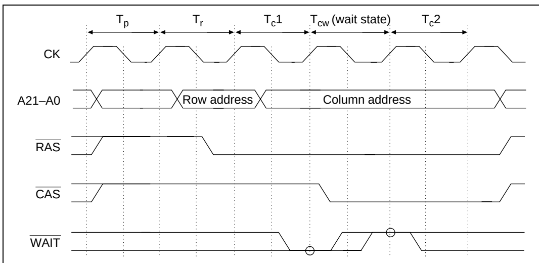
Figure 8.20 Wait State Timing during DRAM Access (Long Pitch)
