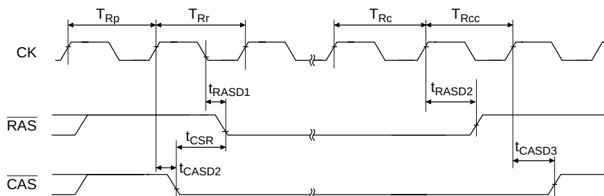
Figure 20.31 Self-Refresh
