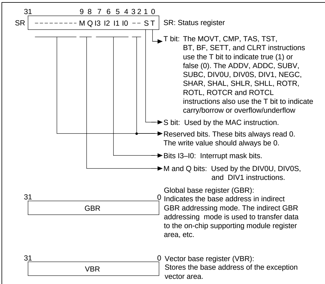
Figure 2.2 Control Registers
