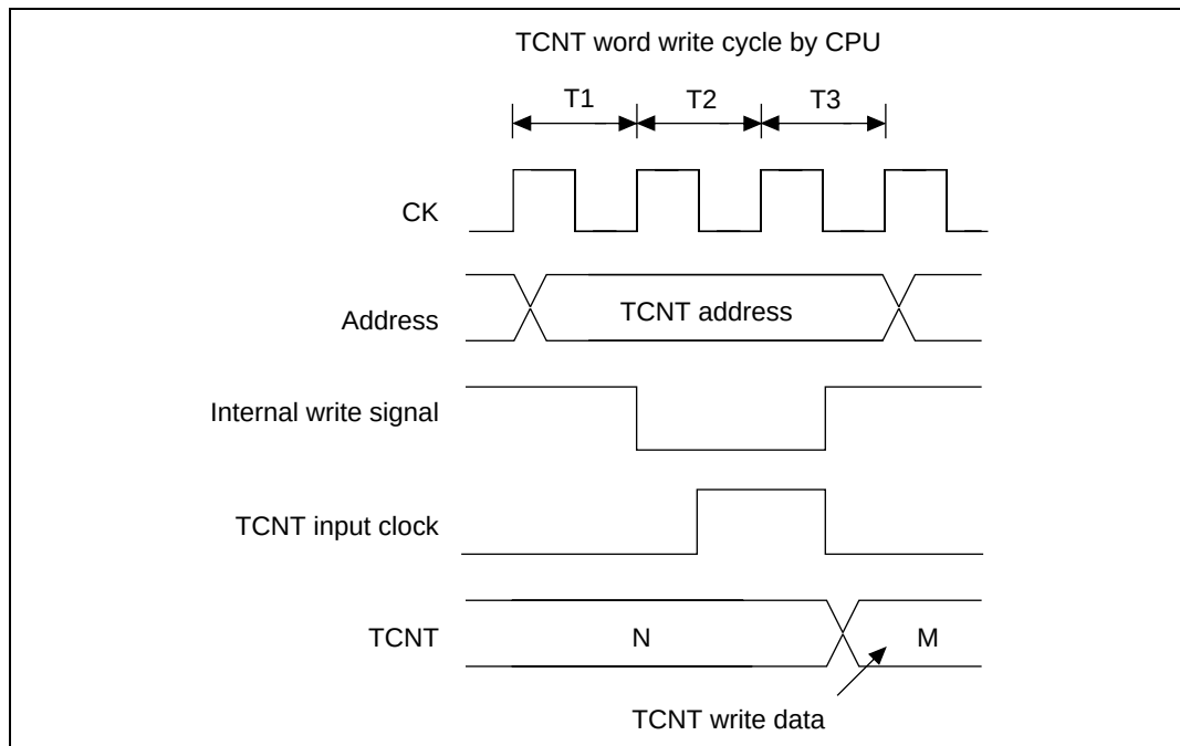
Figure 10.59 Contention between TCNT Word Write and Increment
