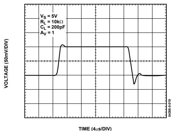
Figure 22. Small Signal Transient
