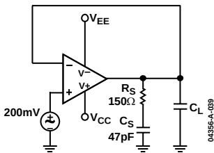
Figure 43. Snubber Network
