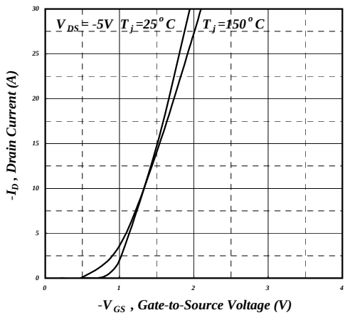
Fig 11. Transfer Characteristics
