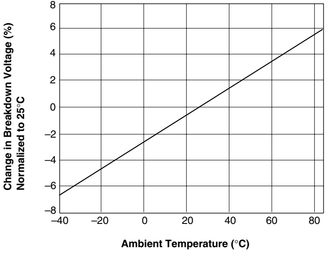
Figure 4. Switch Breakdown Voltage vs. Temperature
