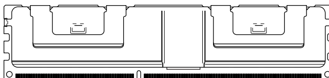
Figure 1: 240-Pin LRDIMM (R/C A) MO-269
