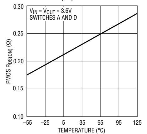
PMOS R_{DS(ON)}
