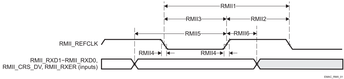
Figure 5-19. EMAC Receive Interface Timing RMI operation
