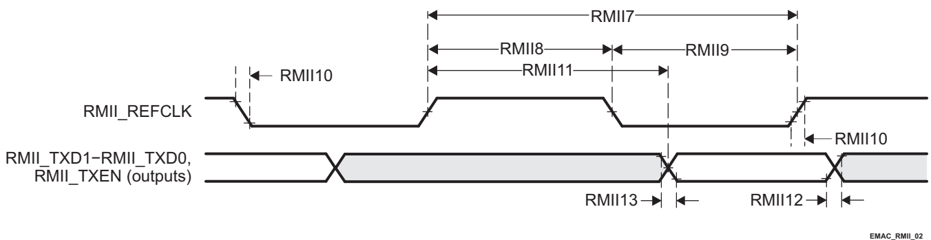
Figure 5-20. EMAC Transmit Interface Timing RMI Operation
