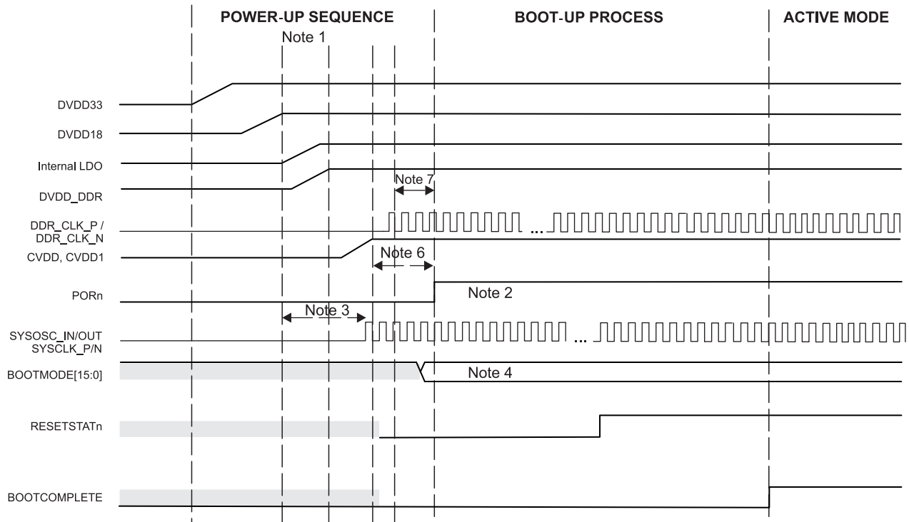
Figure 5-1. Power-Up Sequencing
