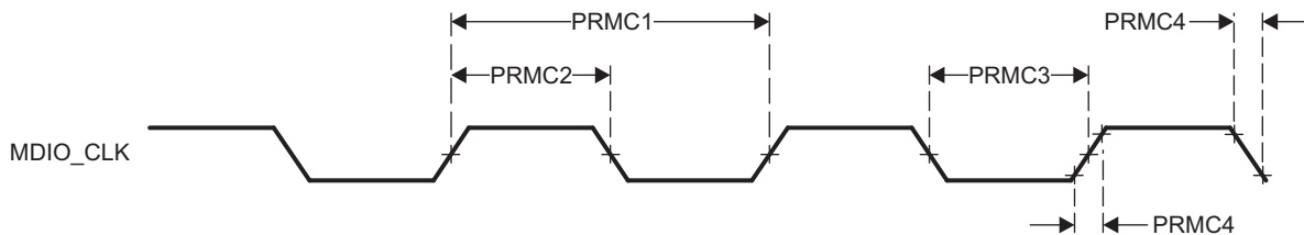
Figure 5-65. PRU-ICSS MDIO_CLK Timing
