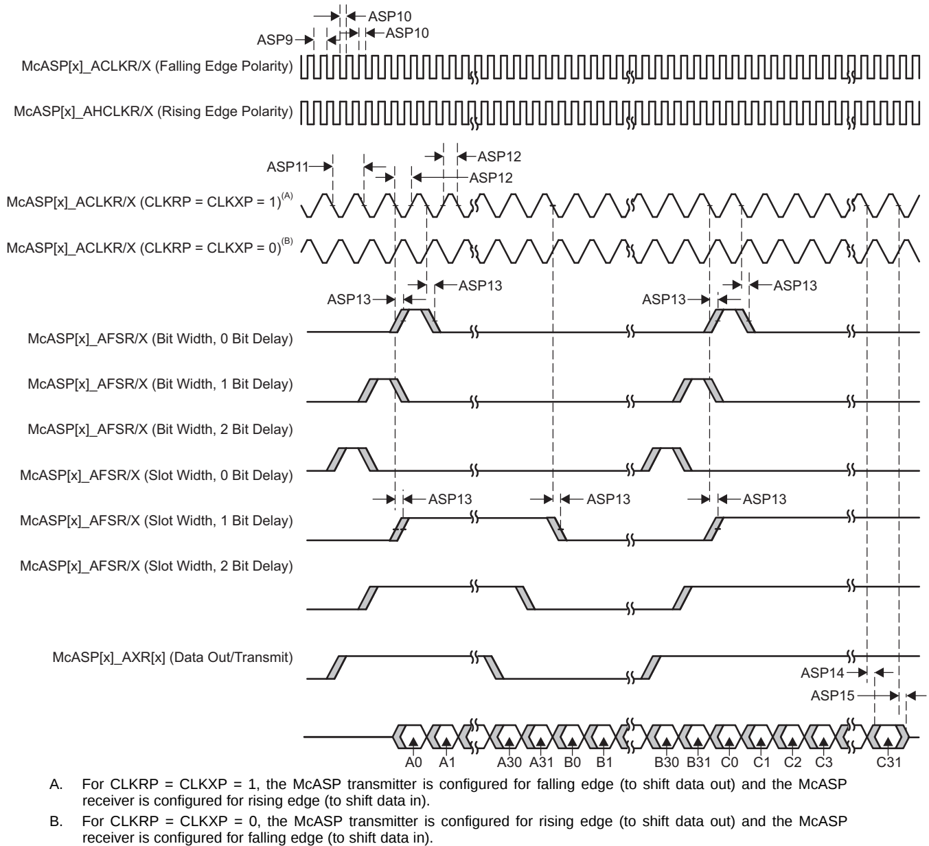
Figure 5-43. McASP Output Timing
