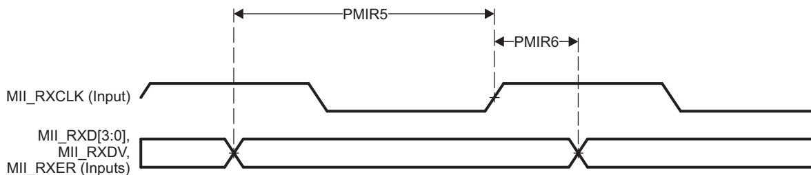
Figure 5-69. PRU-ICSS MII_RXD[3:0], MII_RXDV, and MII_RXER Timing
