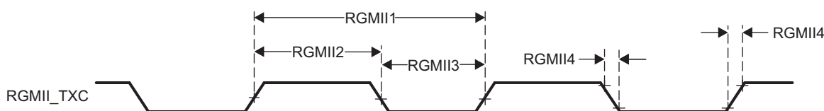
Figure 5-22. RGMII_TCX Timing - RGMII Mode
