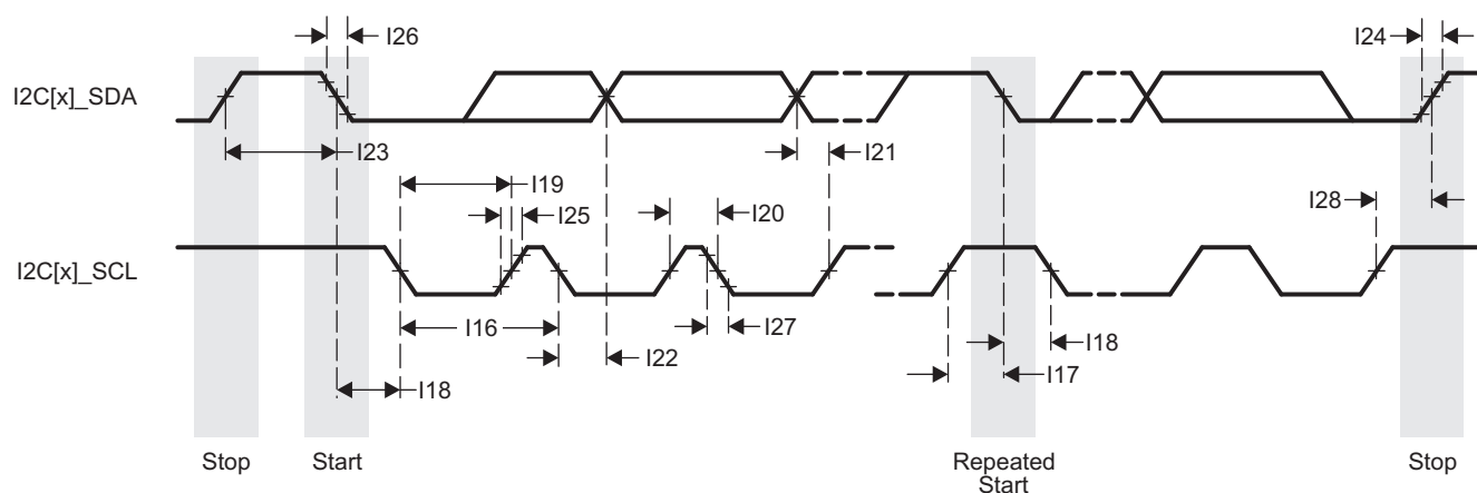
Figure 5-41. I2C Transmit Timing (1)
