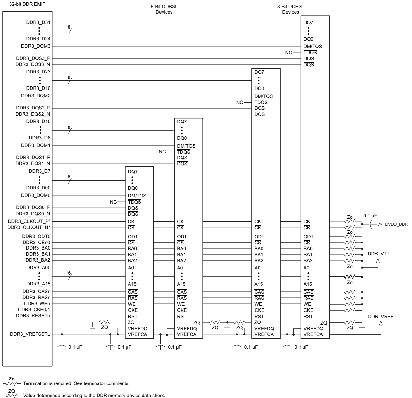
Figure 7-3. 32-Bit, One-Bank DDR EMIF Interface Schematic Using Four 8-Bit DDR3L Devices
