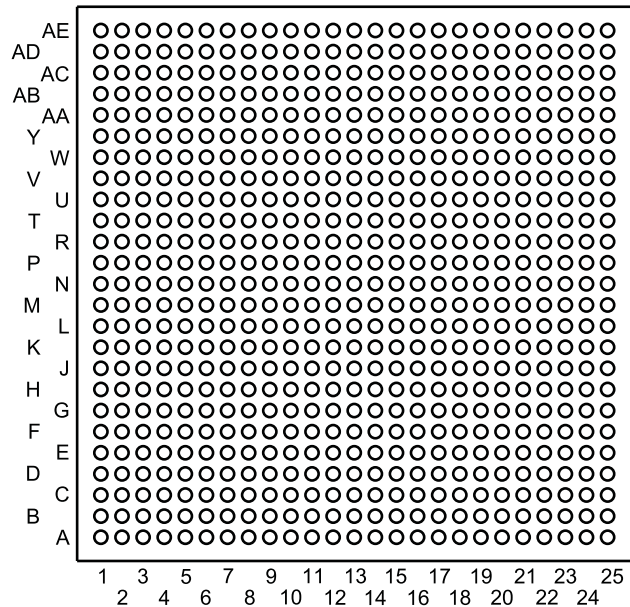
Figure 4-1. ZBB NFBGA-N625 Package (Bottom View)
