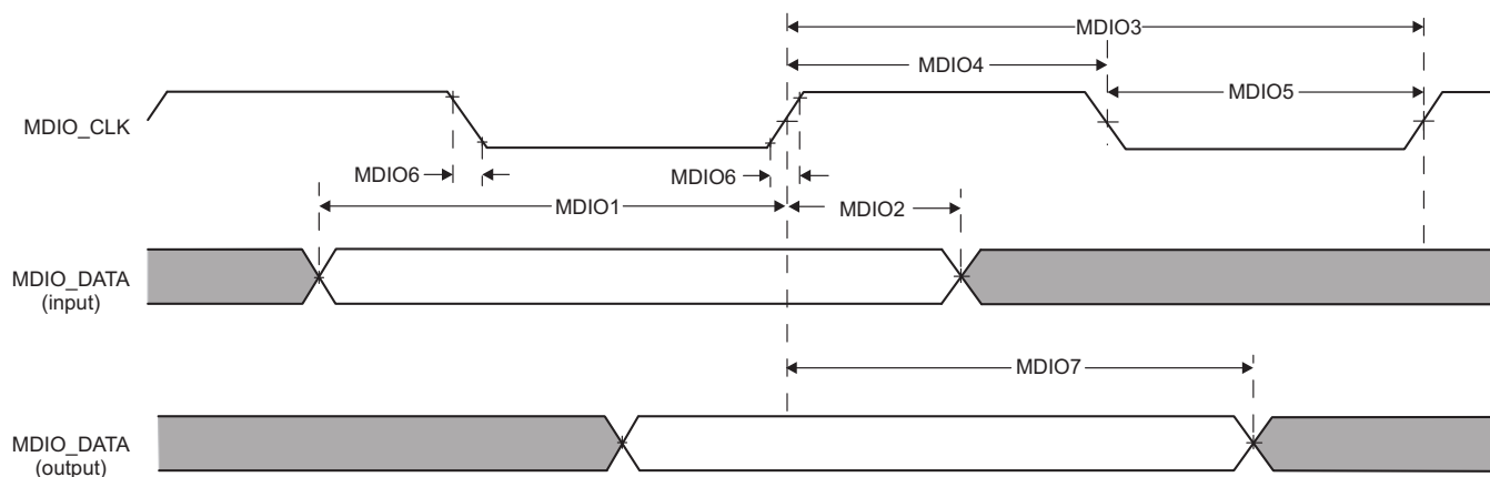
Figure 5-14. EMAC MDIO Diagrams receive and transmit
