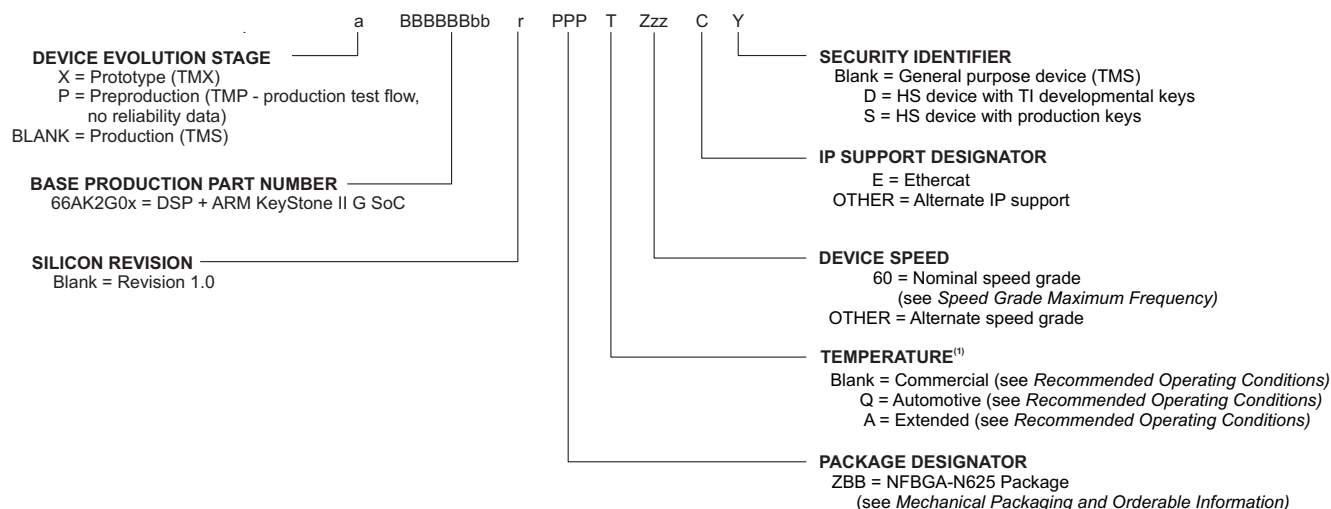
Figure 8-1. Device Nomenclature
