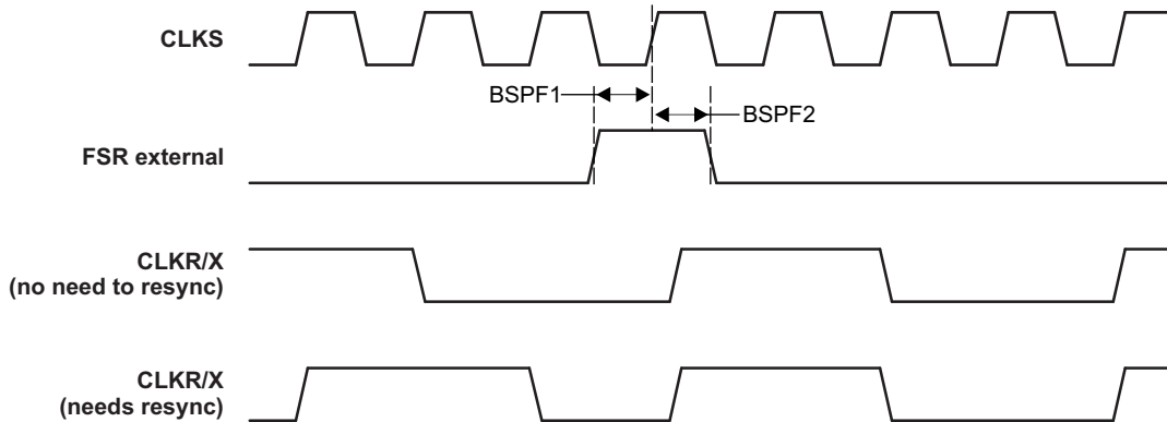
Figure 5-45. FSR Timing When GSYNC = 1
