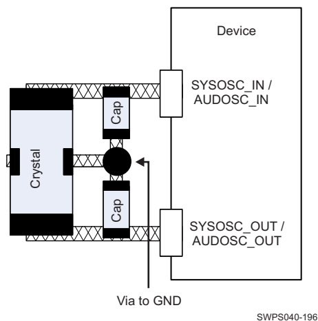
Figure 7-24. SYSOSC and AUDOSC PCB requirements
