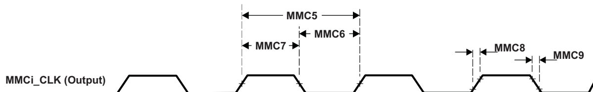
Figure 5-52. MMCi_CLK Timing (1)
