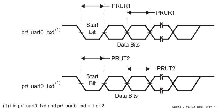
Figure 5-71. PRU-ICSS UART Timing
