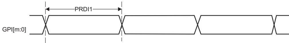
Figure 5-55. PRU-ICSS PRU Direct Input Timing
