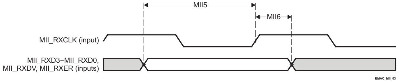
Figure 5-17. EMAC Receive Interface Timing MII operation
