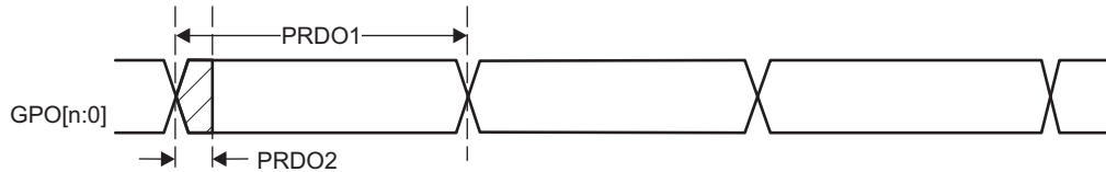
Figure 5-56. PRU-ICSS PRU Direct Output Timing
