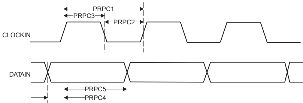
Figure 5-57. PRU-ICSS PRU Parallel Capture Timing – Rising Edge Mode
