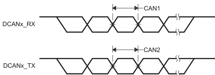
Figure 5-12. DCANx Timings
