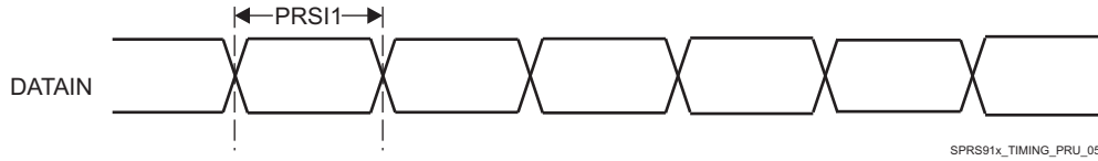
Figure 5-59. PRU-ICSS PRU Shift In Timing
