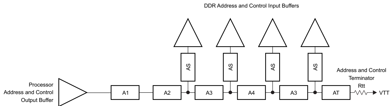
Figure 7-7. ADDR_CTRL Topology for Four x8 DDR3L Devices
