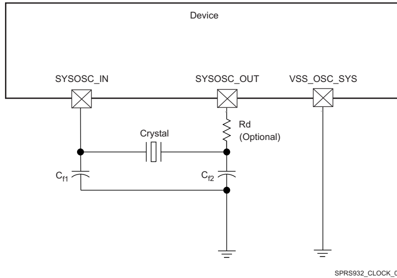
Figure 5-6. Crystal Implementation (1)
