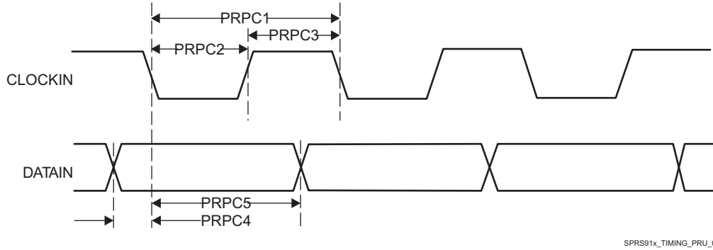
Figure 5-58. PRU-ICSS PRU Parallel Capture Timing – Falling Edge Mode
