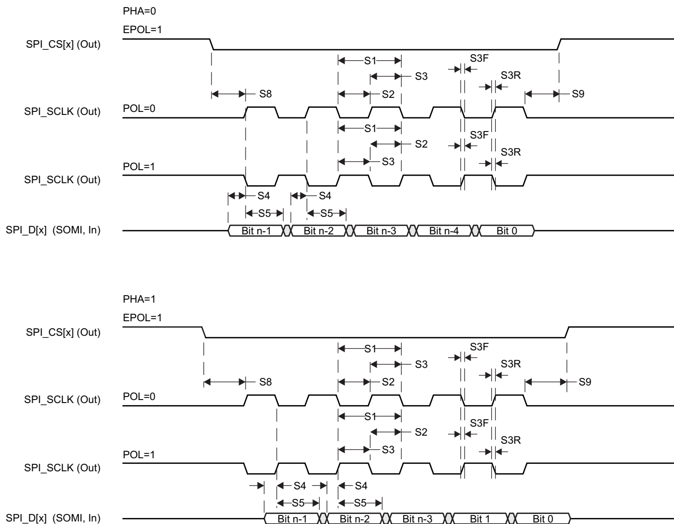
Figure 5-79. SPI Master Mode Receive Timing
