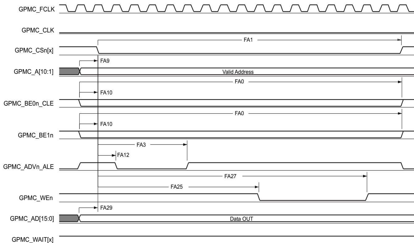
Figure 5-33. GPMC and NOR Flash—Asynchronous Write—Single Word
