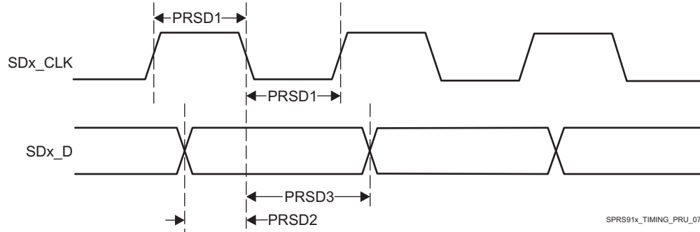
Figure 5-72. PRU-ICSS PRU SD_CLK Falling Active Edge
