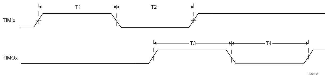
Figure 5-81. Timer Timing
