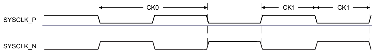
Figure 5-11. SYSCLK_P/N Input Clock
