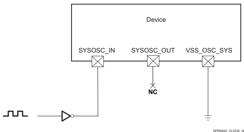
Figure 5-8. LVCMOS-Compatible Clock Input
