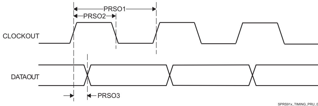
Figure 5-60. PRU-ICSS PRU Shift Out Timing
