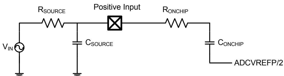
Figure 32-7. ADC Input
