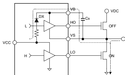
Figure 6. Charging Period
