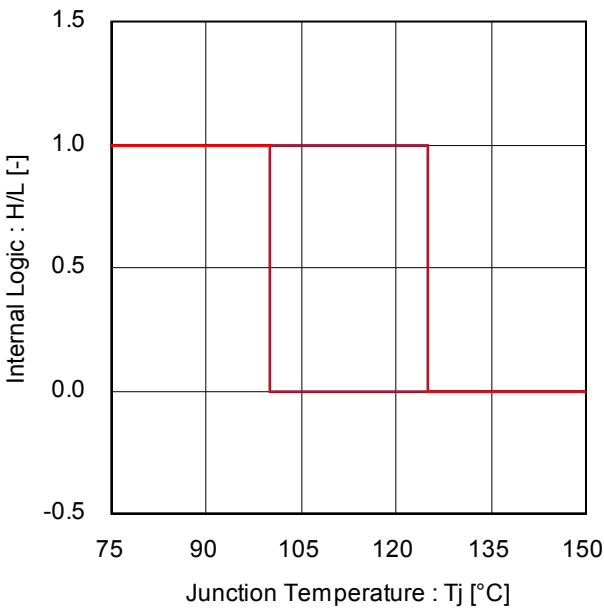
Figure 43. Thermal Shutdown
