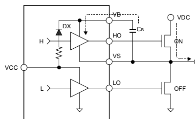
Figure 7. Discharging Period
