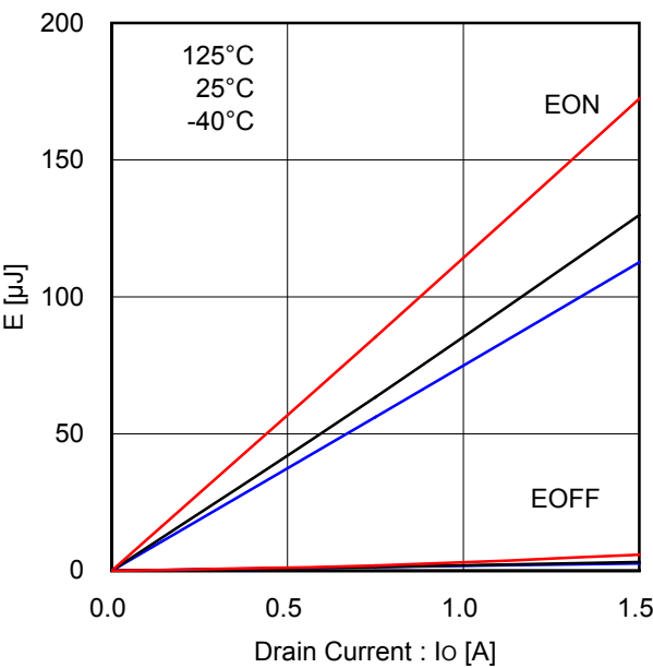
Figure 22. High Side Switching Loss (VDC=300V)
