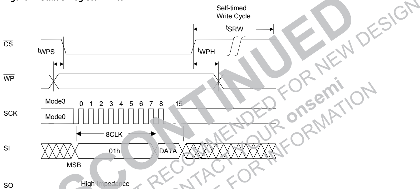
Figure 7. Status Register Write
