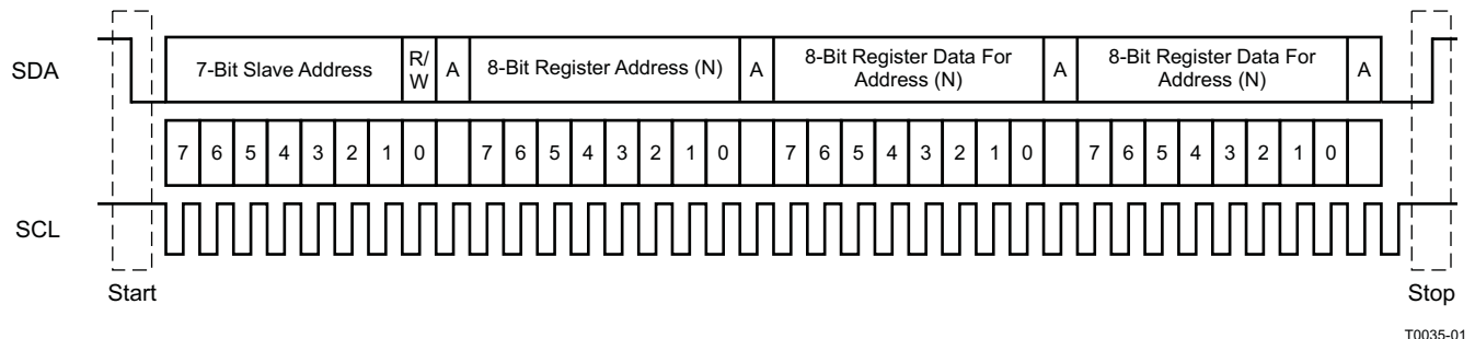
Figure 5-1. Typical I 2 C Sequence
