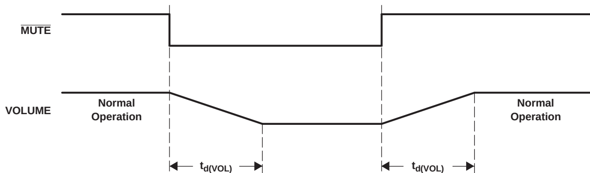
Figure 4-7. Mute Timing
