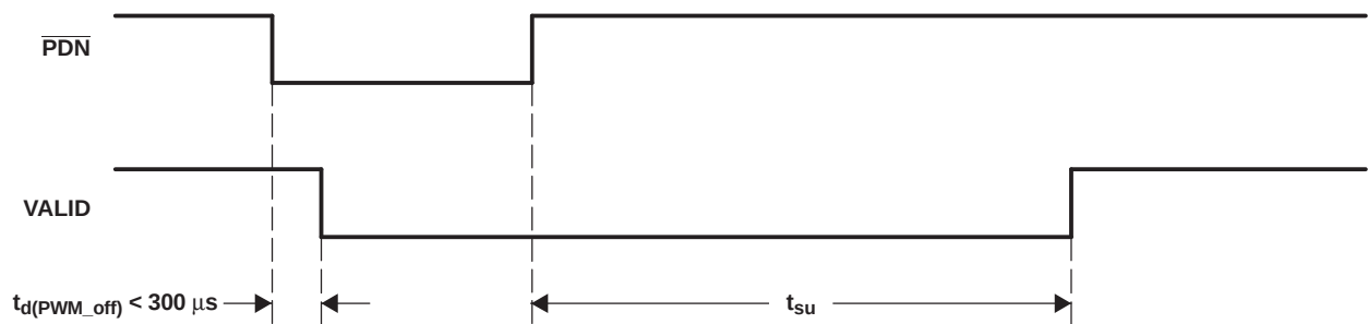
Figure 4-5. Power-Down Timing
