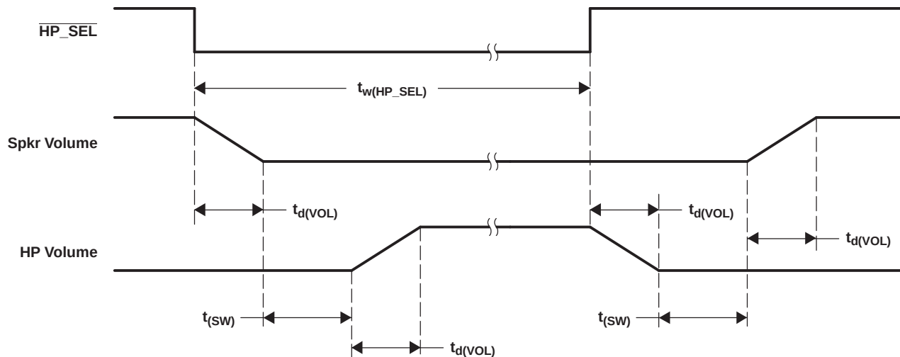
Figure 4-8. \overline{\text{HP\_SEL}} Timing
