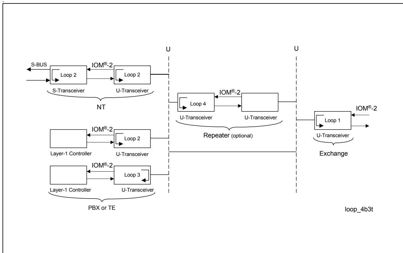
Figure 26 Test Loopbacks
