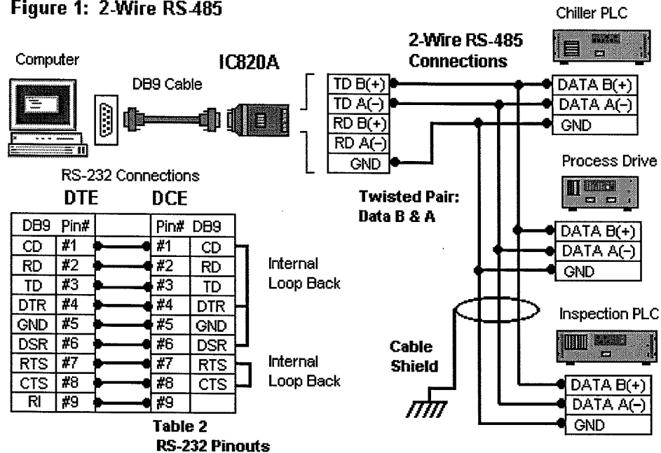
Figure 1: 2-Wire RS-485
